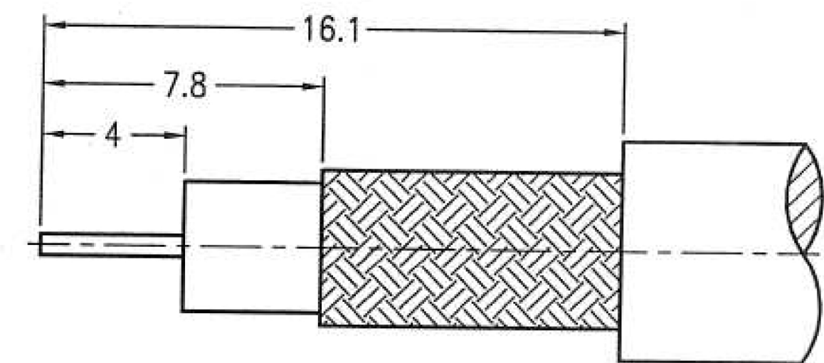
RECOMMENDED CABLE STRIPPING DIM'S
