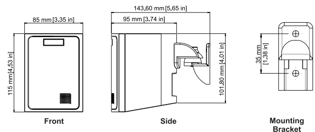
Surface mount satellite speaker and mounting bracket
